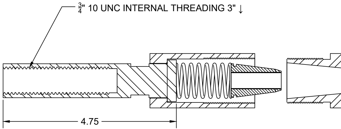
SECTION B-B
